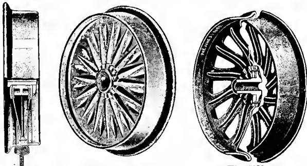
Figs. 5620-5621. THE BUDA CORRUGATED STEEL WHEEL. THE BUDA STEEL WHEEL.* *The Tread and Web of Wheel are formed by Drawing and Spinning a Single Plate of Steel.
